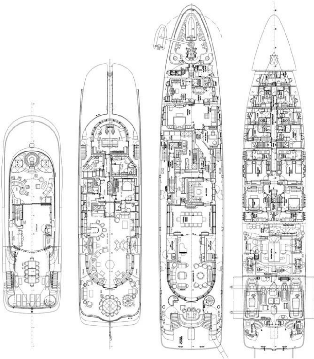
BELLA VITA, 197' (59.90m) Lurssen Motoryacht, 2010/2024
